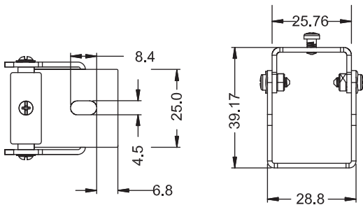
Angle Adjustable Bracket
