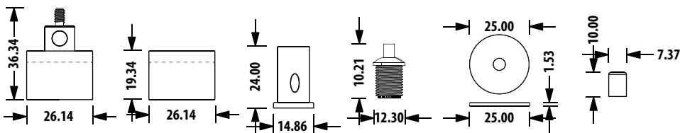
DIY Pendant Accessories Connector Kit
