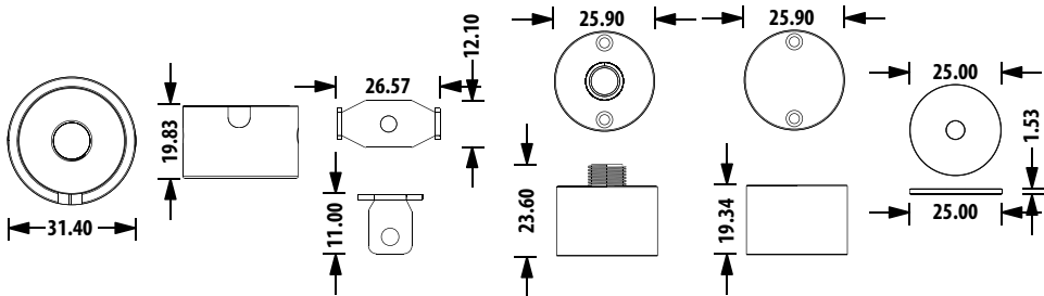
DIY Pendant Accessories Connector Kit
