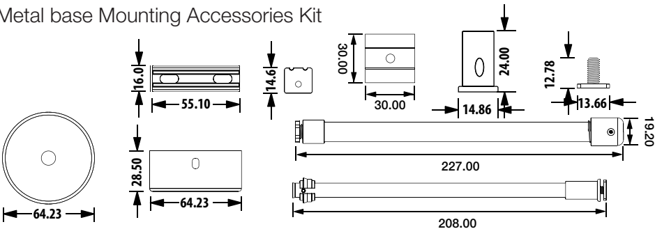
Aluminum alloy base Mounting Accessories Kit
