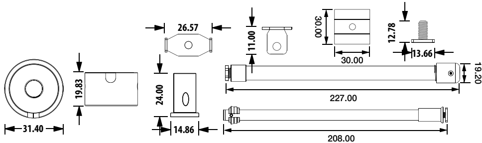
Aluminum alloy base Mounting Accessories Kit
