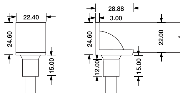
Bottom Entry Connector
