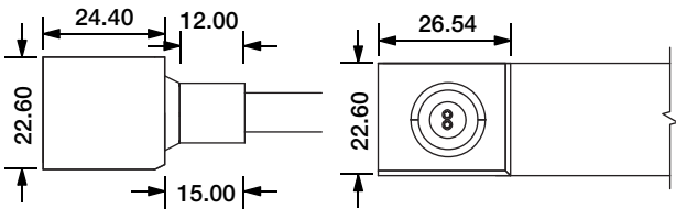
Bottom Entry Connector
